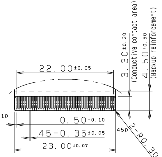
Detail B (S=2/1)
