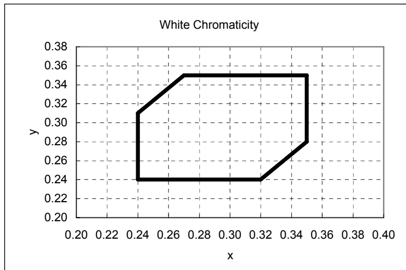
Fig. 4: White Chromaticity Range
