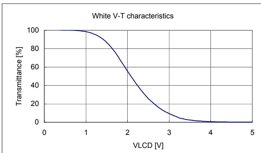
Fig. 3: White V-T Curve
